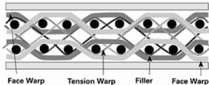
Solid Woven Carcass
